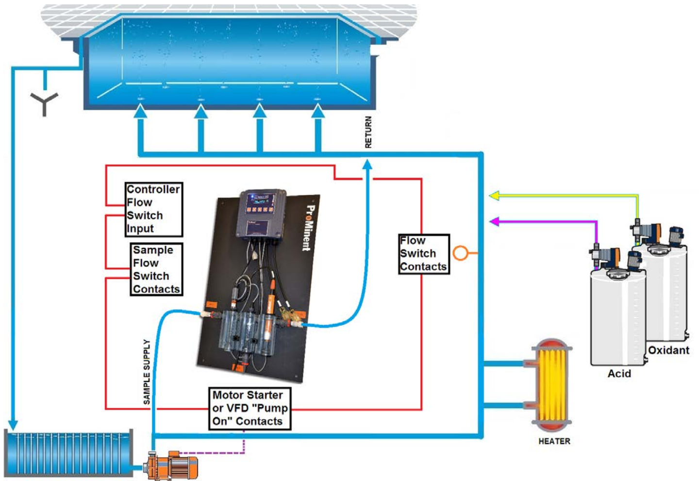
DCM2 safety interlock connections for vacuum filter systems
