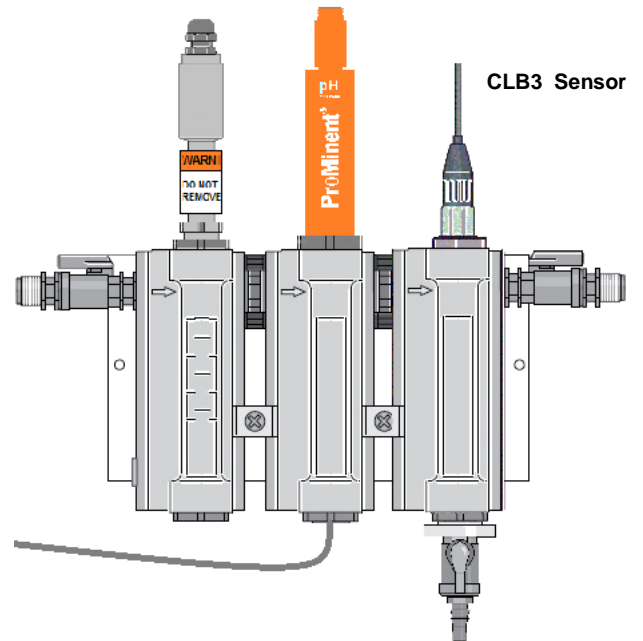
DCM2-CI Sensor Arrangement
