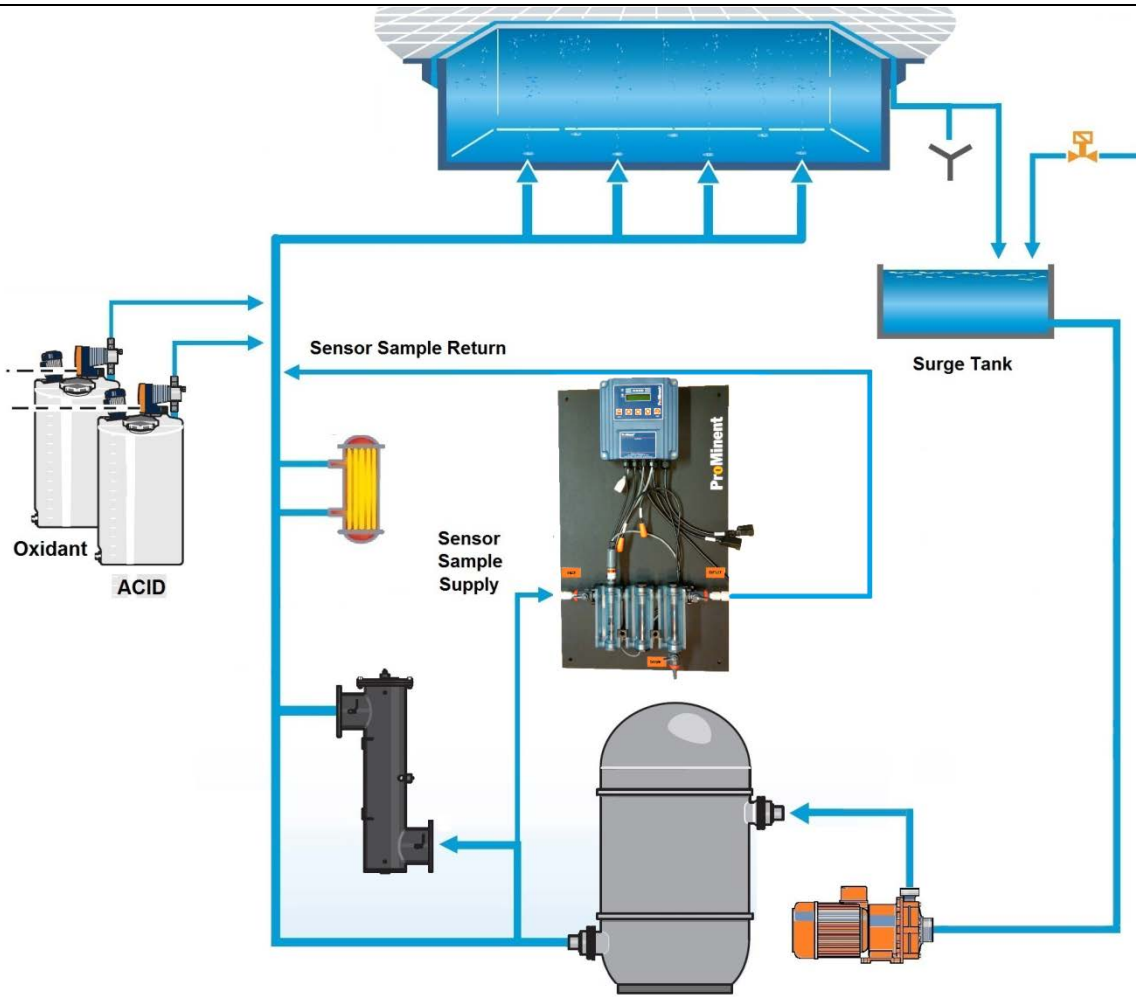
Proper Pressure Filter Arrangement
