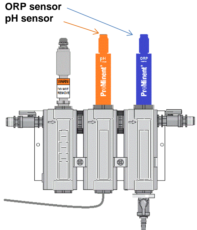
DCM200 Sensor Arrangement
