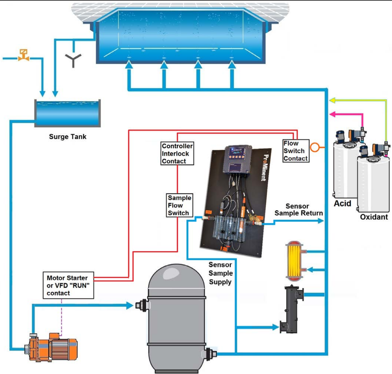
DCM2 safety interlock connections for pressure filter systems
